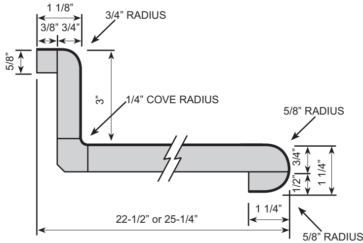
KITCHEN & VANITY TOP ETV-22 1/2 ETK-25 1/4
